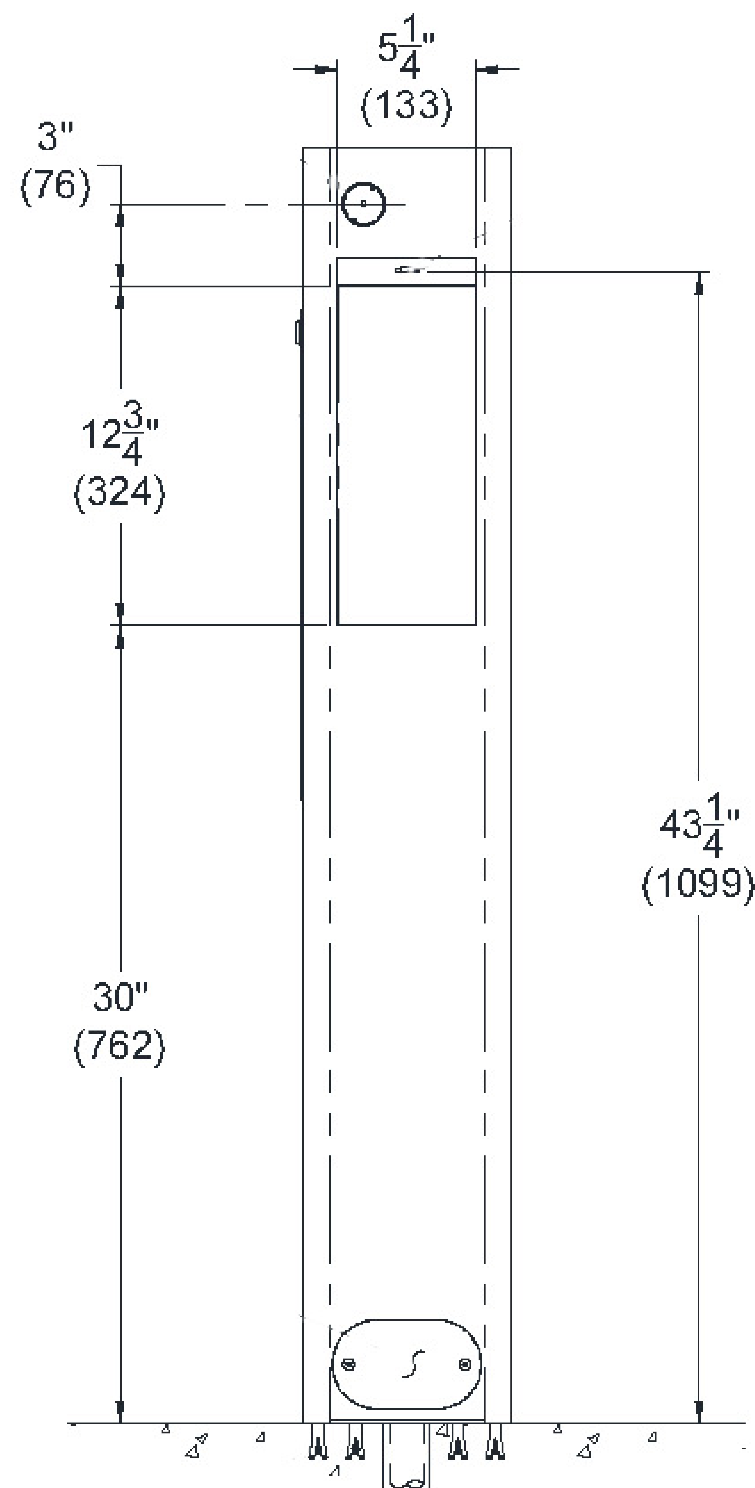
FRONT VIEW
