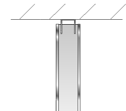
5 Wall connection with an U-profile as a shadow gap
