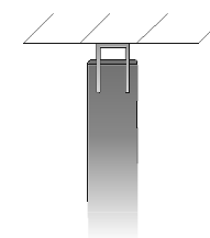
5 Wall connection with an U-profile as a shadow gap
