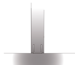
3 Front to partition wall connection
