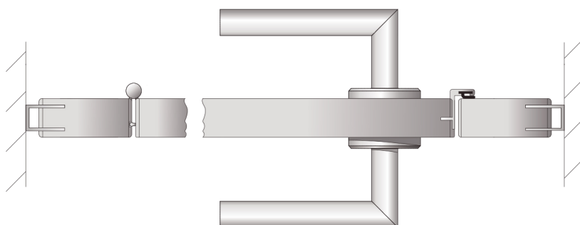
2 Cubicle front section with with door handle
