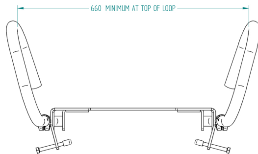
SPLAYED HANDLE POSITION
